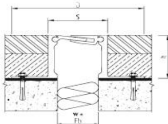
PAV 23-50 h=70
